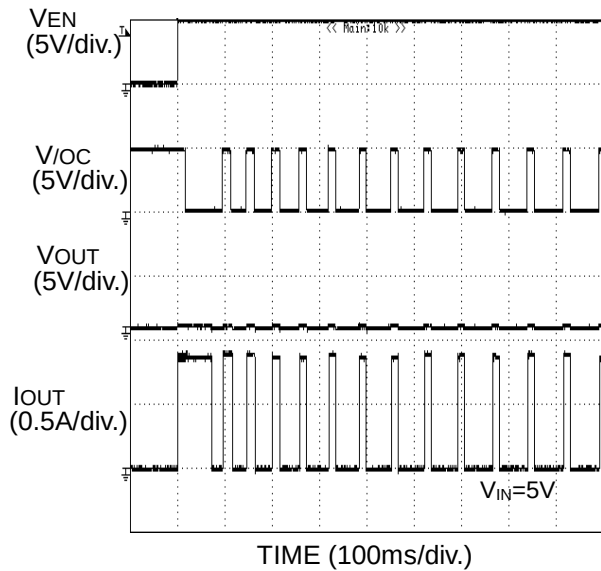
Figure 35. Over-Current Response Enable to Short Circuit
