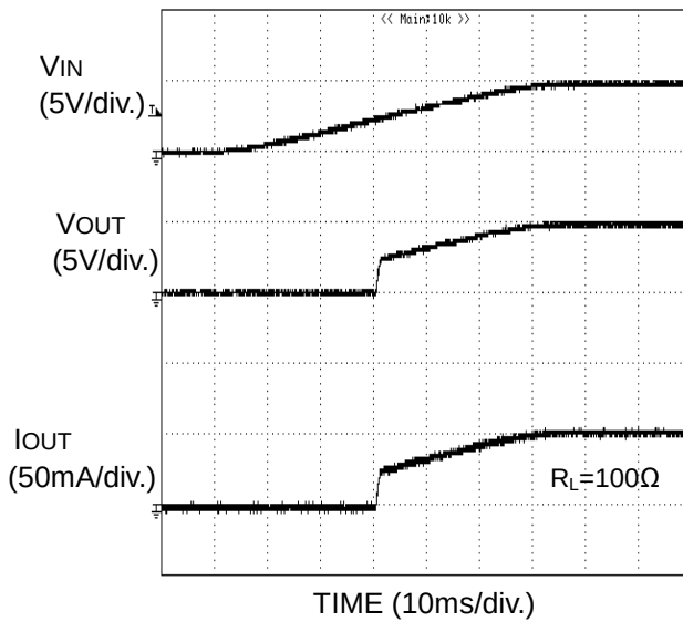
Figure 37. UVLO Response when Increasing VIN
