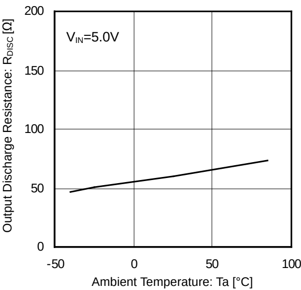
Figure 29. Output Discharge Resistance vs Ambient Temperature
