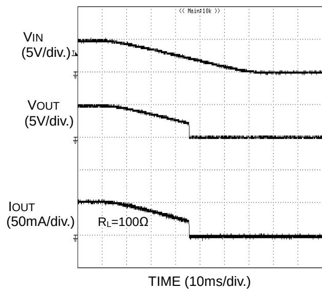
Figure 38. UVLO Response when Decreasing V_{IN}
