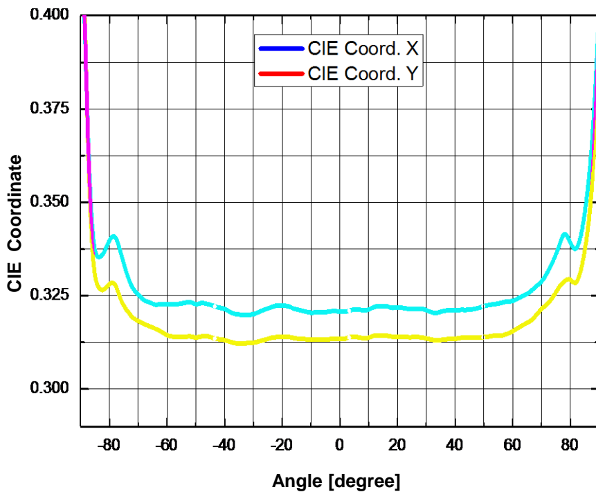
Fig 10. Color vs. Viewing Angle, I_F = 20\text{mA} , T_j = 25^\circ\text{C}
