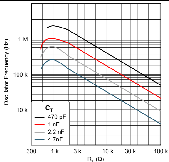
Figure 6. Oscillator Frequency vs Timing Resistance
