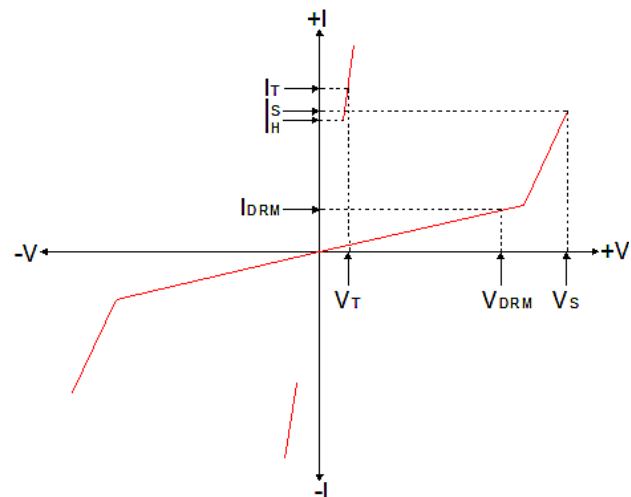
V-I Curve
