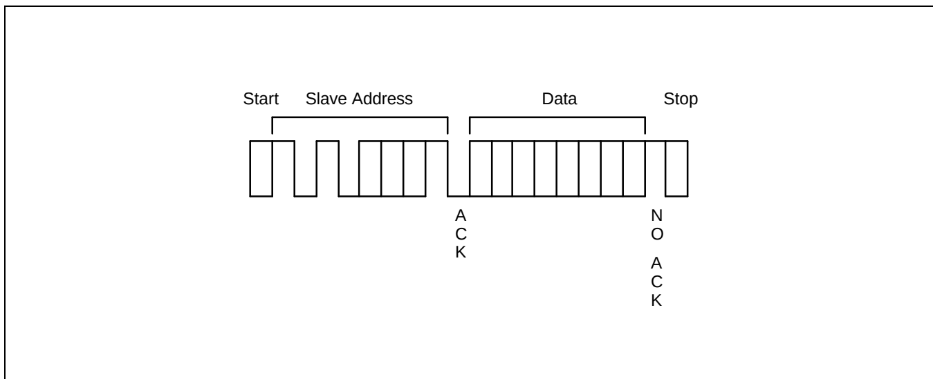
Figure 7-13. Current Address Byte Read Operation
