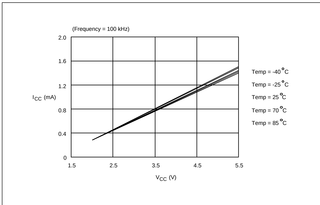
Figure 7-18. Write Current
