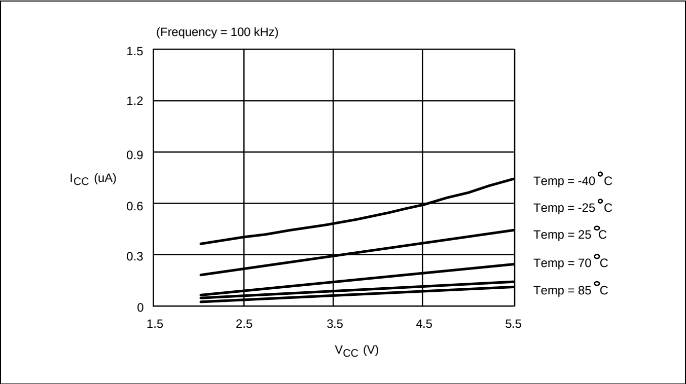
Figure 7-20. Stand-by Current
