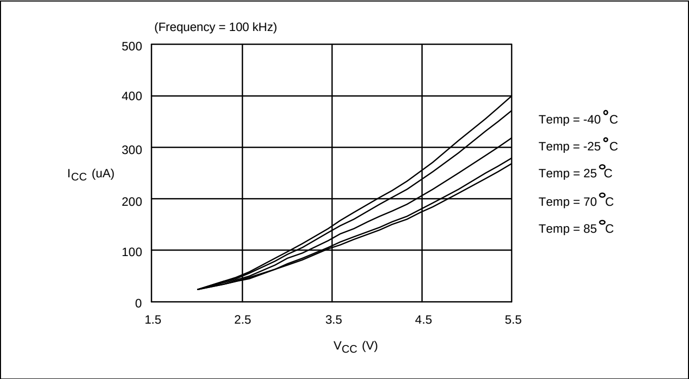
Figure 7-19. Read Current
