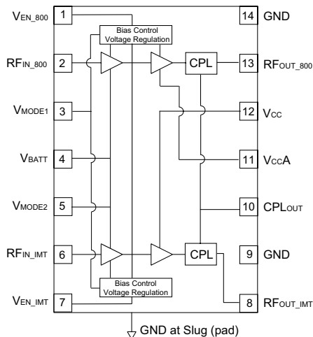
Figure 1: Block Diagram
