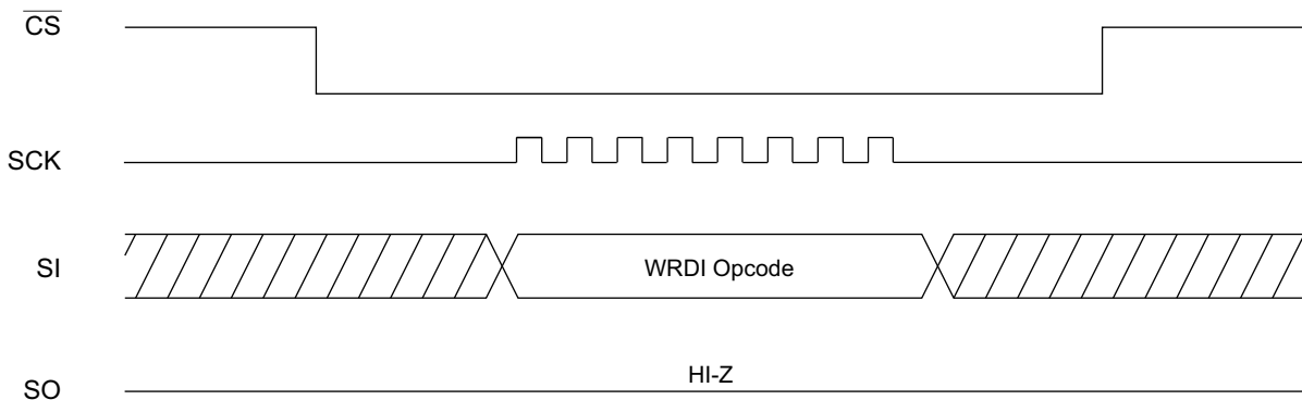
Figure 6-3. WRDI Timing
