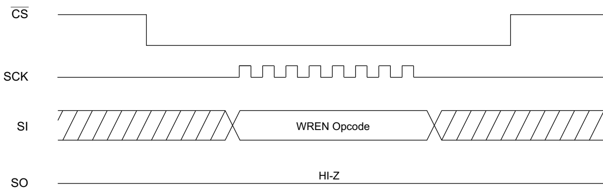
Figure 6-2. WREN Timing
