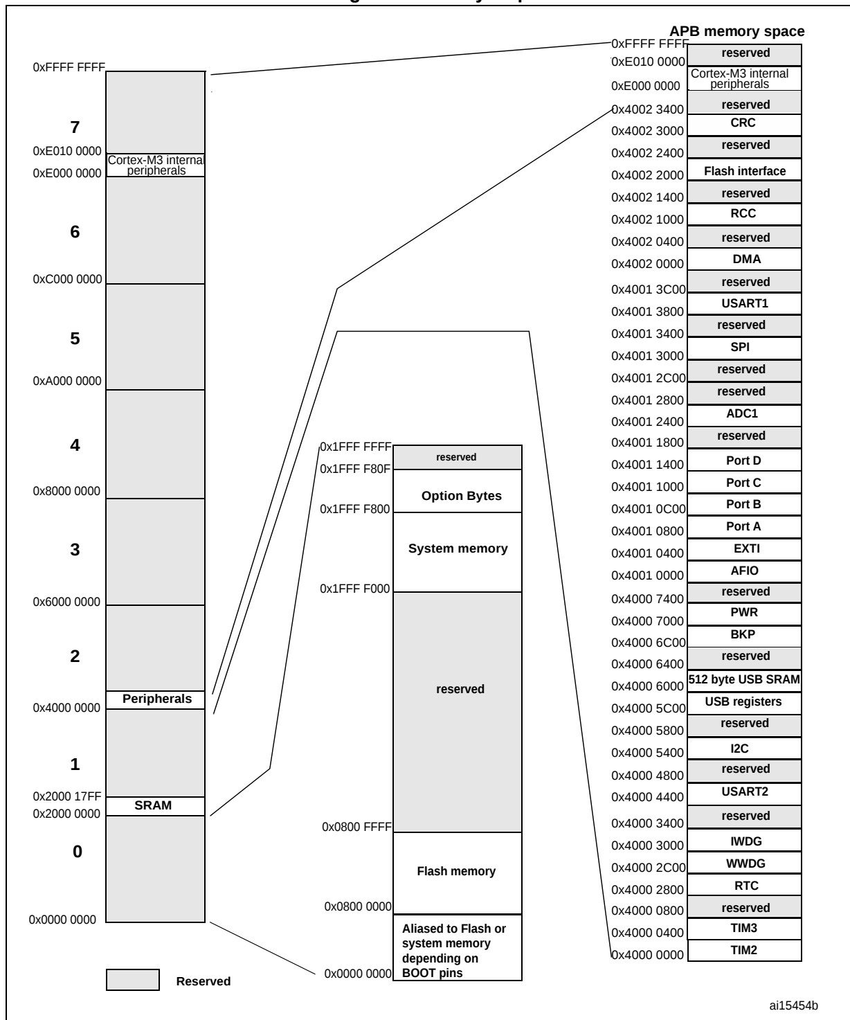
Figure 5. Memory map
