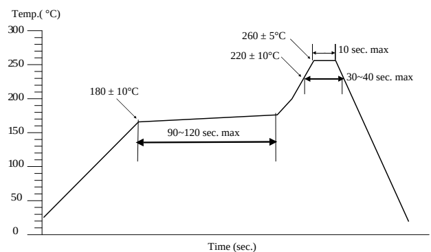
Reflow profile
