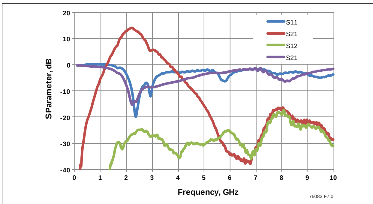
FIGURE 6-7: RECEIVER S-PARAMETER
