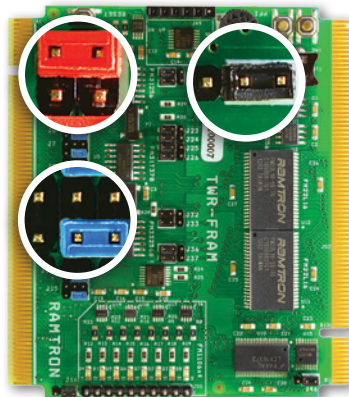
6-pin jumper
