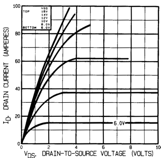
Fig 16. Typical Output Characteristics Post-Irradiation 1 Mega Rads (Si)
