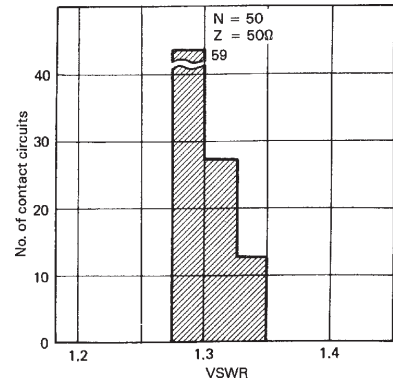
Distribution of VSWR at 900 MHz
