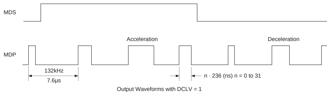
Timing Chart 1-14
