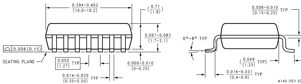
14-Lead Small Outline Package EIAJ Package Number M14D
