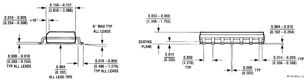
14-Lead (0.150" Wide) Small Outline Integrated Circuit Package Number M14A
