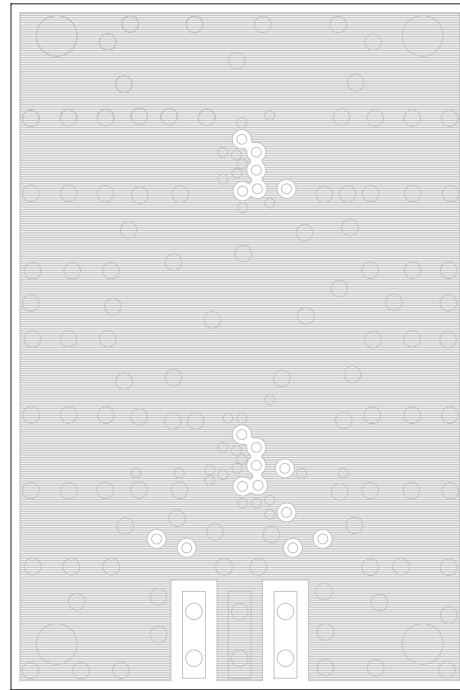
Layer 2: Ground
