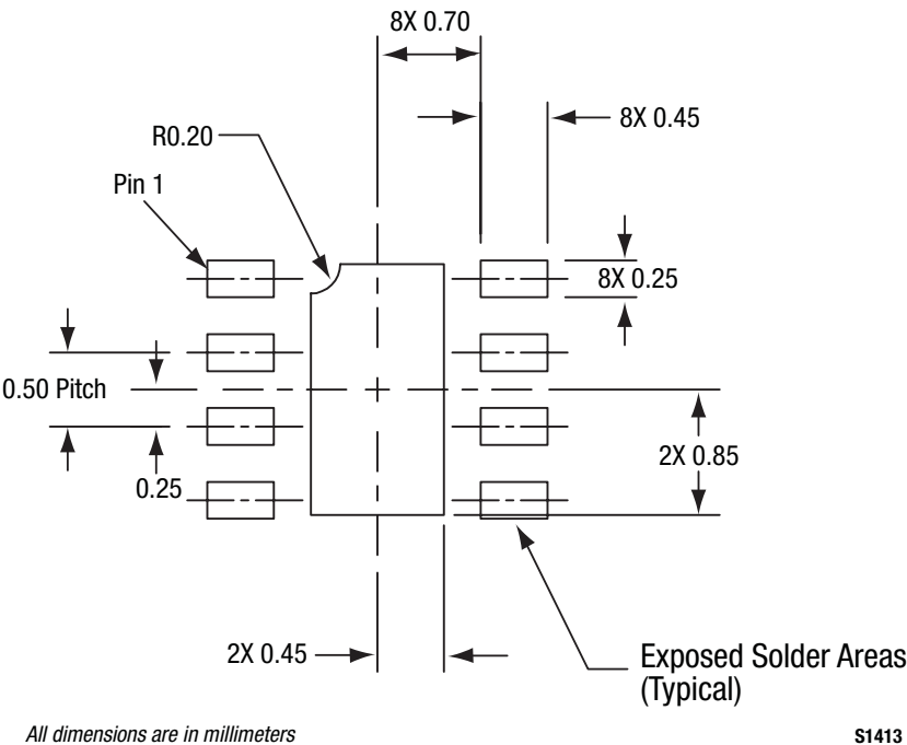
Figure 20. SKY65047-360LF PCB Layout Footprint
