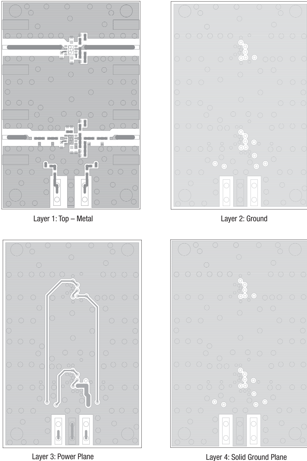
Figure 16. SKY65047-360LF Evaluation Board Layer Detail (915 MHz)
