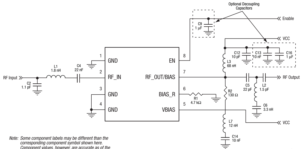
Figure 14. SKY65047-360LF Evaluation Board Schematic (2450 MHz)
