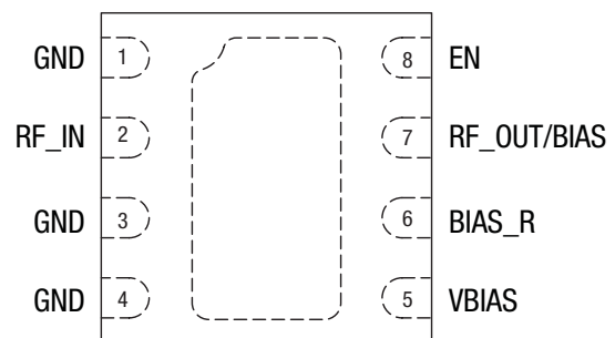
Figure 2. SKY65047-360LF Pinout – 8-Pin QFN (Top View)
