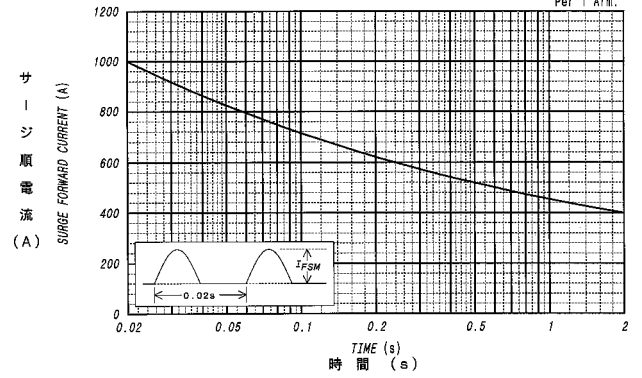
サージ順電流定格 SURGE CURRENT RATINGS f=50Hz, Half Sine Wave, Non-Repetitive, T_j=150^\circ\text{C}
