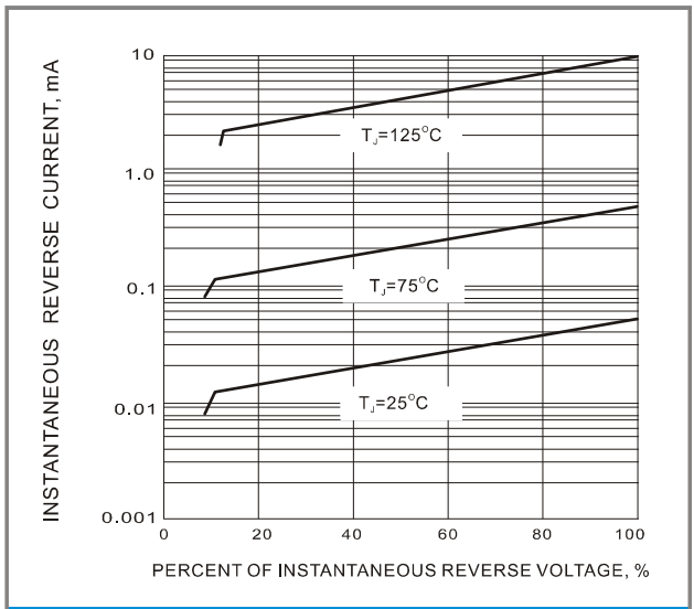
Fig.3-TYPICAL REVERSE CHARACTERISTIC
