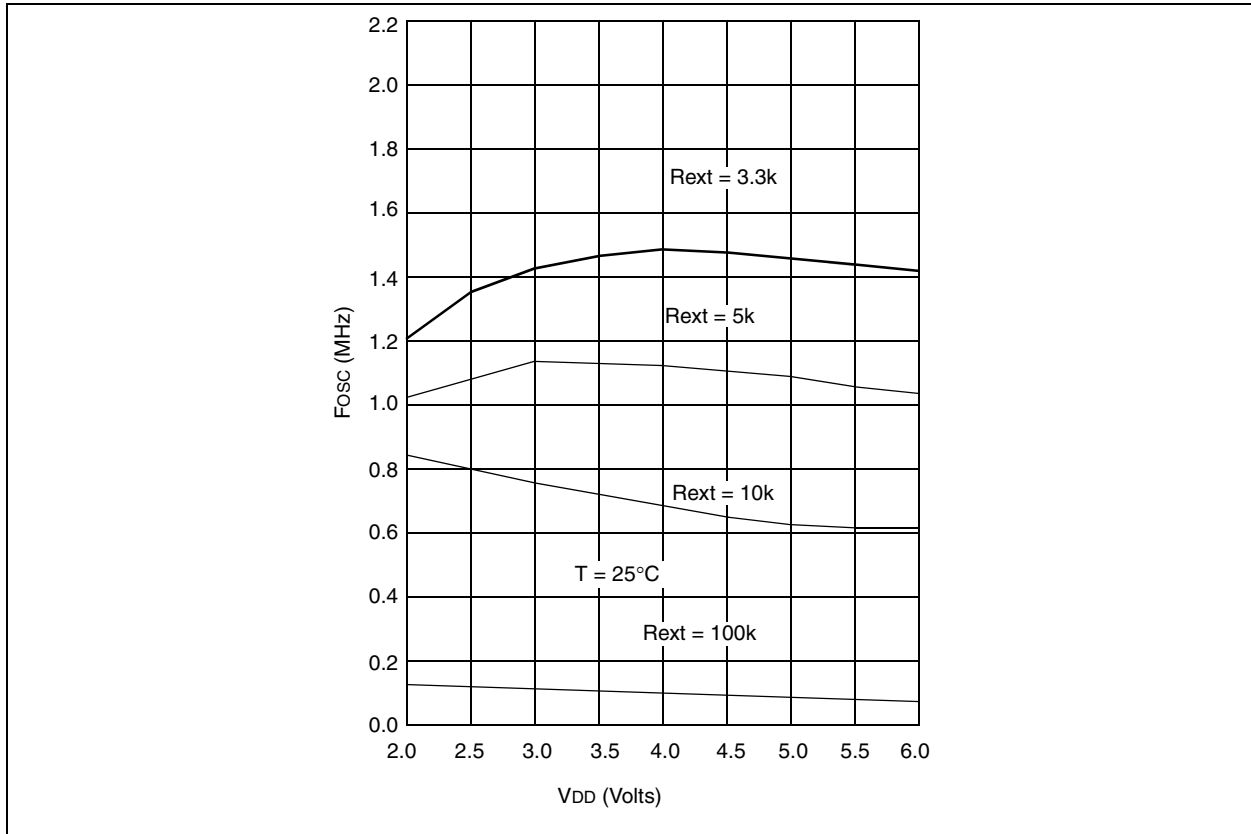
FIGURE 12-3: TYPICAL RC OSCILLATOR FREQUENCY vs. V_{DD} ( C_{ext} = 100\text{ pF} )
