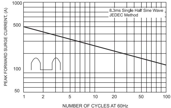
FIG.2- MAXIMUN NON-REPETITIVE PEAK FORWARD SURGE CURRENT
