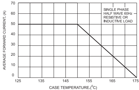
FIG.1- MAXIMUN FORWARD CURRENT DERATING CURVE
