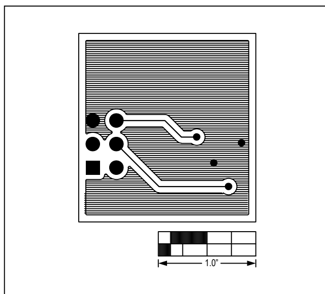
Figure 15. MAX44006 Daughter Board PCB Layout—Bottom
