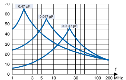
Suppression versus frequency. Typical values.
