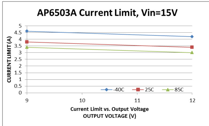
Figure 4. Typical Overcurrent Performance with V_{IN} = 15V
