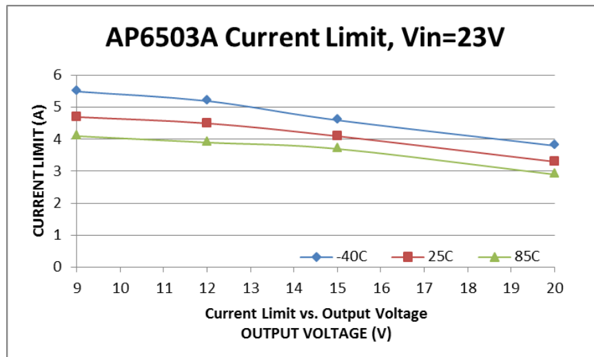
Figure 6. Typical Overcurrent Performance with V_{IN} = 23V
