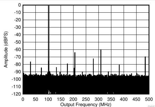
Low power mode, F_S = 1000 MSPS Figure 7-14. Single Tone FFT at 897 MHz and -1 dBFS
