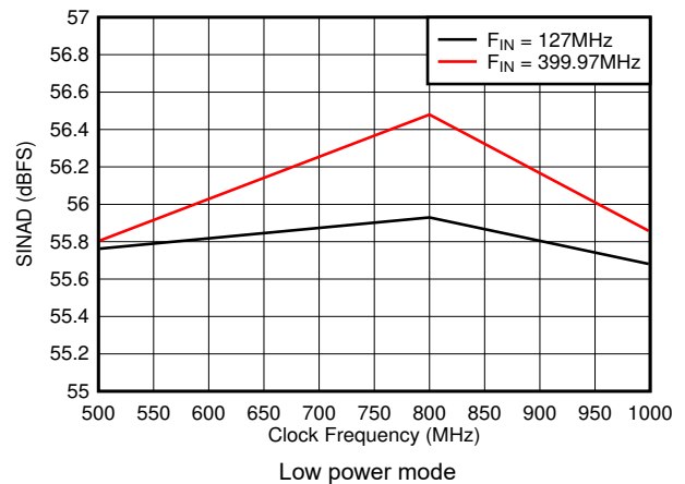
Figure 7-30. SINAD vs Sample Rate
