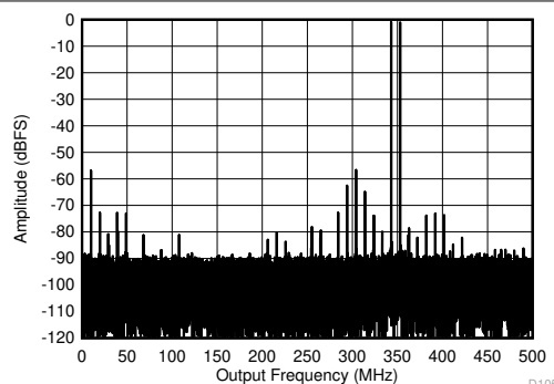
Figure 7-70. Two Tone FFT at 1798MHz
