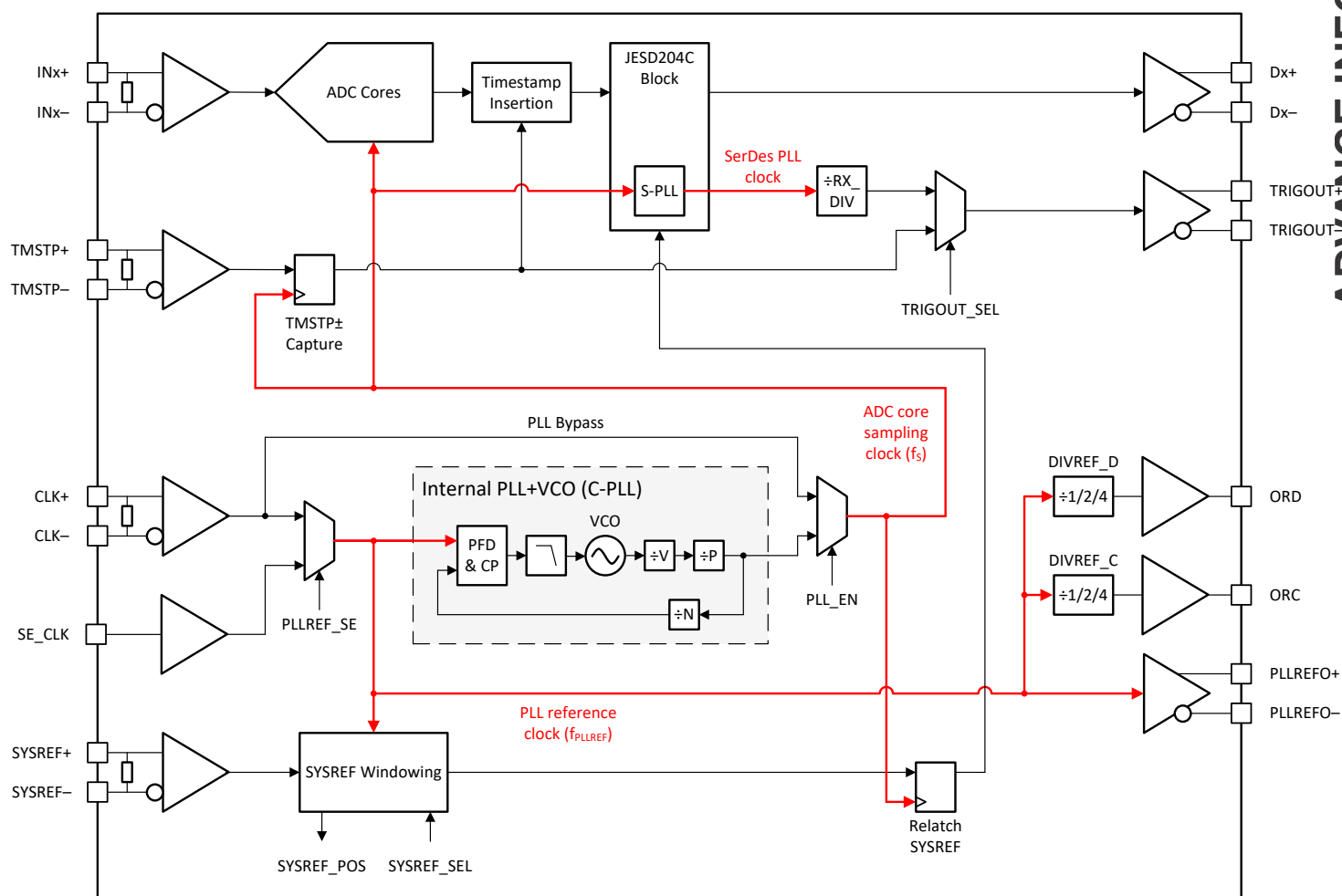
Figure 8-3. Clocking Subsystem
