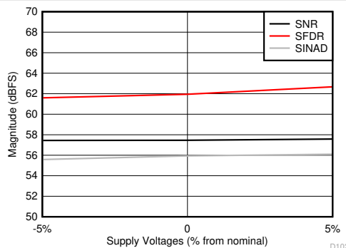
Figure 7-62. SNR, SFDR and SINAD vs Supply Voltages
