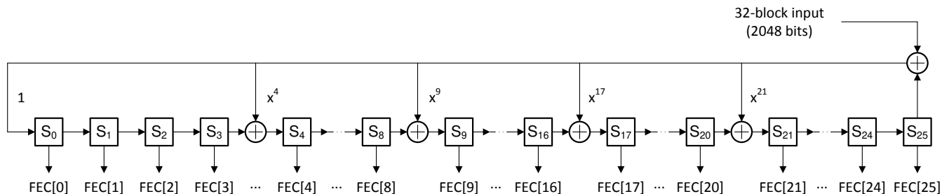
Figure 8-8. FEC Parity Bit Generator
