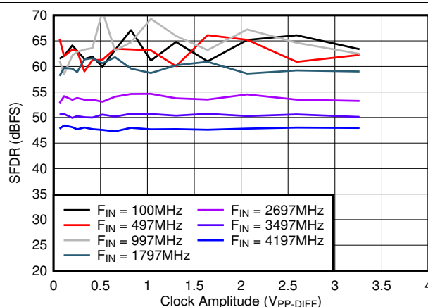
Figure 7-36. SFDR vs A_{CLK}
