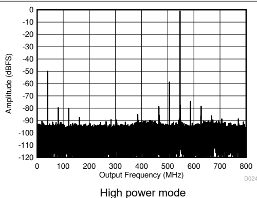
Figure 7-11. Single Tone FFT at 3797 MHz and -1 dBFS
