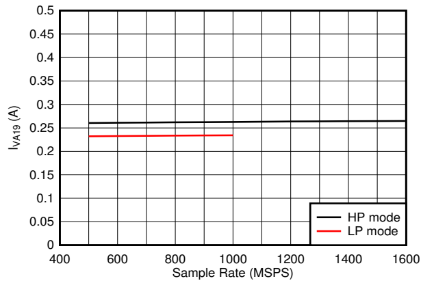
Figure 7-103. Single Channel, I_{VA19} vs F_S
