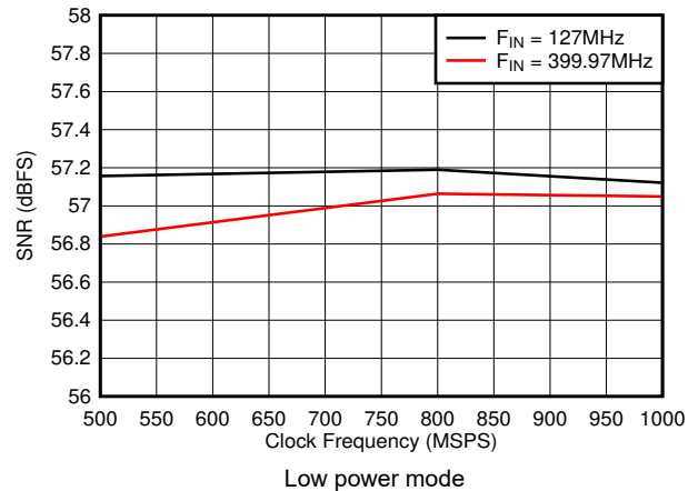
Figure 7-28. SNR vs Sample Rate
