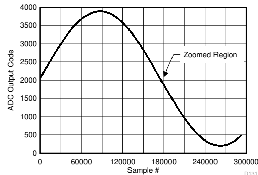
Figure 7-126. Background Calibration Core Transition (AC Signal)
