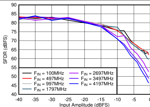
Figure 7-32. SFDR vs A_{IN}
