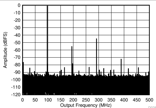
Low power mode, F_S = 1000 MSPS Figure 7-15. Single Tone FFT at 2097 MHz and -1 dBFS
