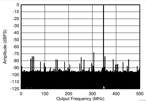
C-PLL on, Low power mode, F_S = 1000 MSPS Figure 7-13. Single Tone FFT at 347 MHz and -1 dBFS
