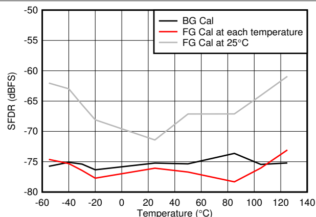
Figure 7-68. Worst Spur vs Temperature
