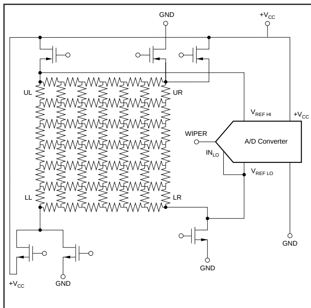
FIGURE 4. Simplified Diagram of Differential Reference ( \text{SER}/\overline{\text{DFR}} LOW).
