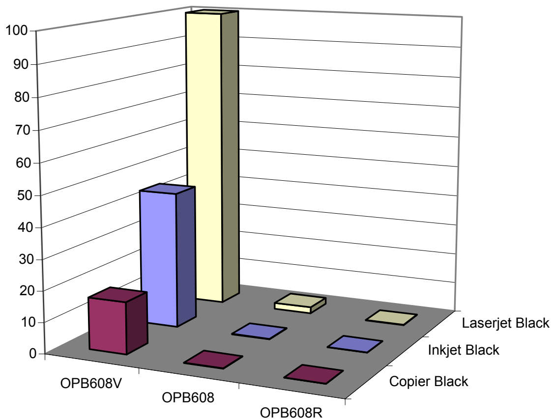
Relative Response
