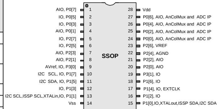
Figure 6. CY8C23433 28-Pin PSoC Device
