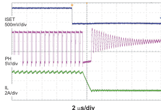
图 8-4. Charge Disable by ISET
