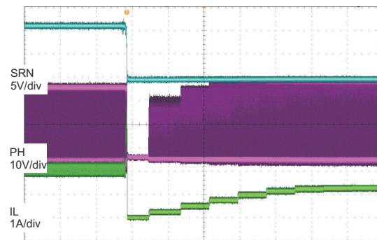
图 8-10. Battery to Ground Short Protection
