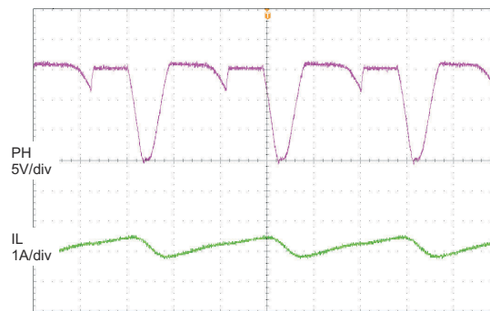
图 8-6. Discontinuous Conduction Mode Switching
