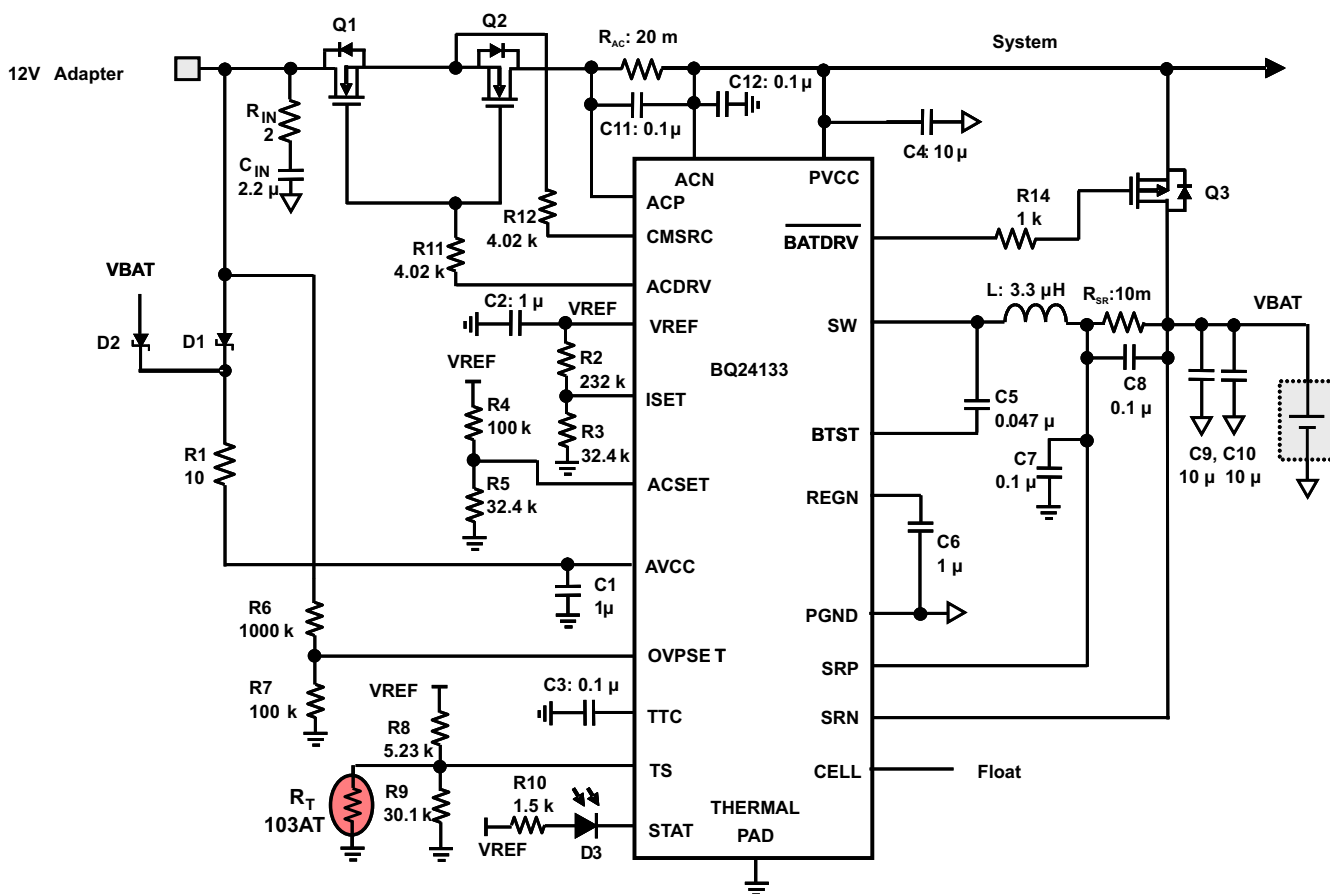
图 10-1. Typical Application Schematic
