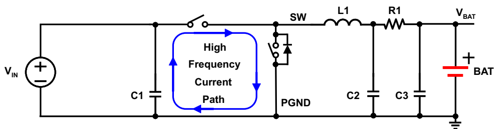
图 12-1. High-Frequency Current Path
