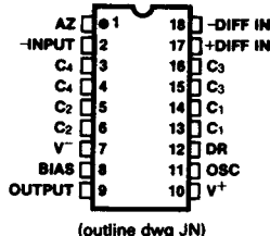
Figure 1: Pin Configuration
