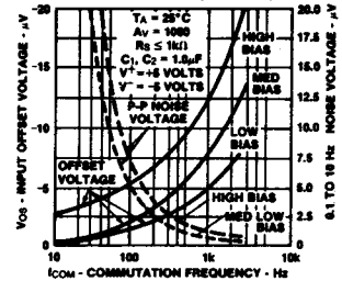
INPUT OFFSET VOLTAGE AND PK-TO-PK NOISE VOLTAGE AS A FUNCTION OF COMMUTATION FREQUENCY ( C_1, C_2 = 1\mu F )
