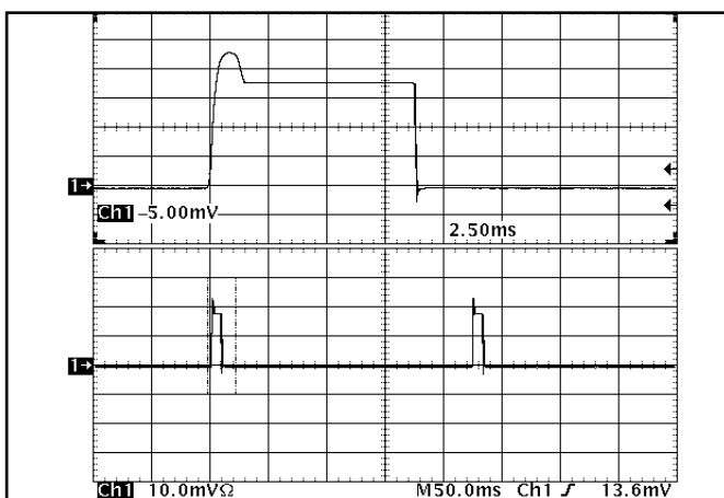
Figure 18: Load current ( 10\ \text{A}/\text{div} ) as a function of time when the converter attempts to turn on into a 10\ \text{m}\Omega short circuit. Top trace ( 2.5\ \text{ms}/\text{div} ) is an expansion of the on-time portion of the bottom trace.
