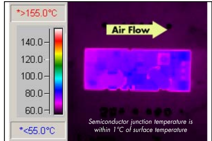
Figure 8: Thermal plot of converter at 15 amp load current with 55 ^{\circ} C air flowing at the rate of 200 LFM. Air is flowing across the converter from input to output (nominal input voltage).
