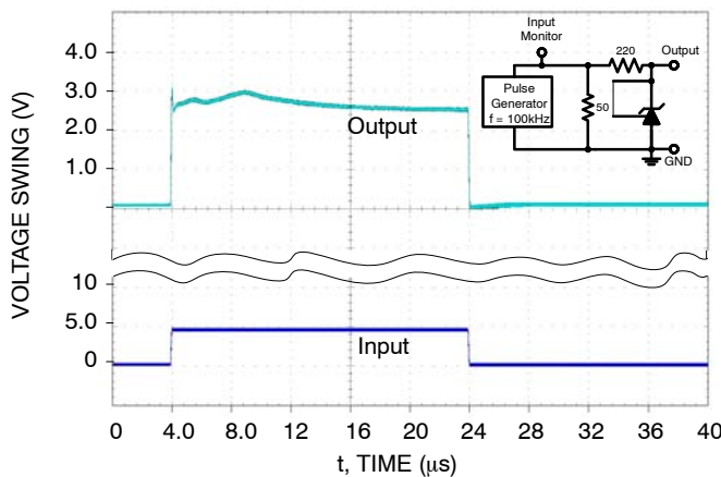
Figure 17. Pulse Response
