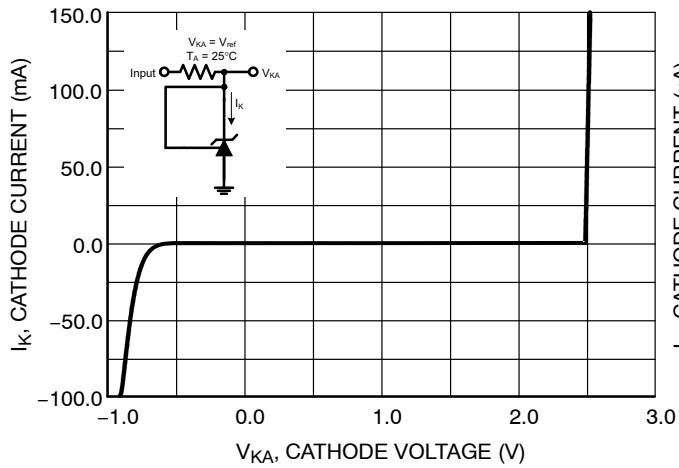
Figure 6. Cathode Current versus Cathode Voltage
