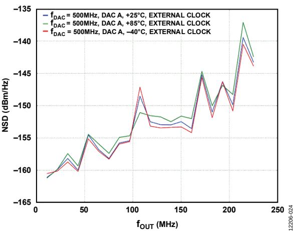
Figure 19. NSD at Three Temperatures vs. f_{OUT}
