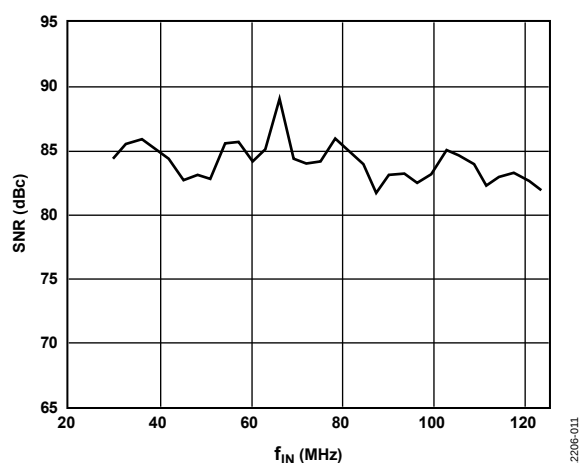
Figure 8. Single Tone SNR vs. Input Frequency ( f_{\text{IN}} )
