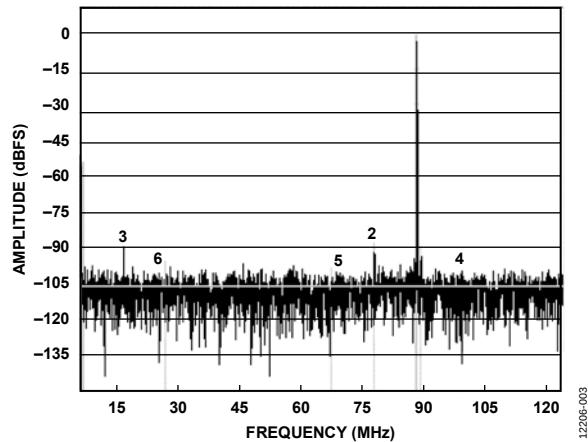
Figure 3. Single Tone FFT, f_{\text{IN}} = 87 \text{ MHz}
