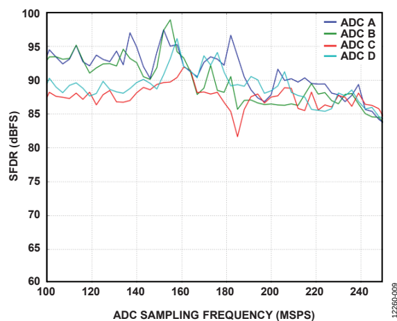
Figure 11. Single Tone SFDR vs. ADC Sampling Frequency ( f_{\text{ADC}} ), f_{\text{IN}} = 90.0 \text{ MHz} , All Four ADCs
