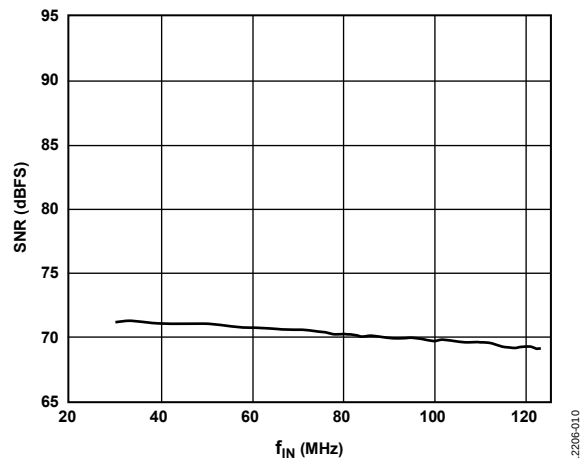
Figure 7. Single Tone SNR vs. Input Frequency ( f_{\text{IN}} )
