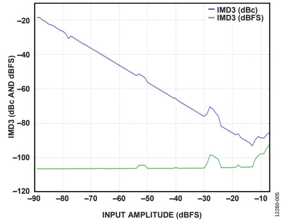
Figure 6. Two Tone IMD3 vs. Input Amplitude ( A_{\text{IN}} ), f_{\text{IN1}} = 89.12 \text{ MHz} , f_{\text{IN2}} = 92.12 \text{ MHz}
