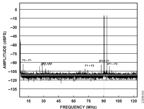
Figure 9. Two Tone FFT, f_{\text{IN1}} = 89.12 \text{ MHz} , f_{\text{IN2}} = 92.12 \text{ MHz}
