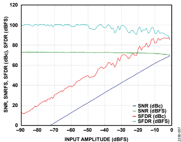
Figure 4. Single Tone SNR and SFDR vs. Input Amplitude ( A_{\text{IN}} ), f_{\text{IN}} = 87 \text{ MHz}
