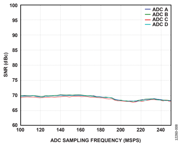
Figure 10. Single Tone SNR vs. ADC Sampling Frequency ( f_{\text{ADC}} ), f_{\text{IN}} = 90.0 \text{ MHz} , All Four ADCs
