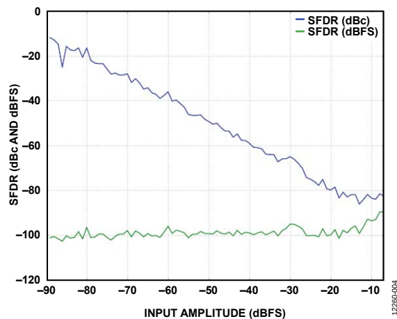
Figure 5. Two Tone SFDR vs. Input Amplitude ( A_{\text{IN}} ), f_{\text{IN1}} = 89.12 \text{ MHz} , f_{\text{IN2}} = 92.12 \text{ MHz}
