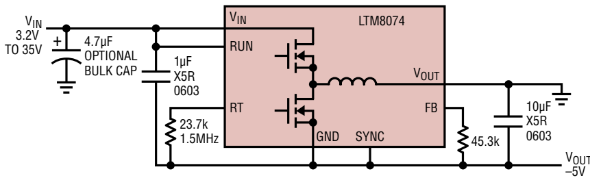
-5V OUT from 3.2V IN to 35V IN Positive to Negative Converter
