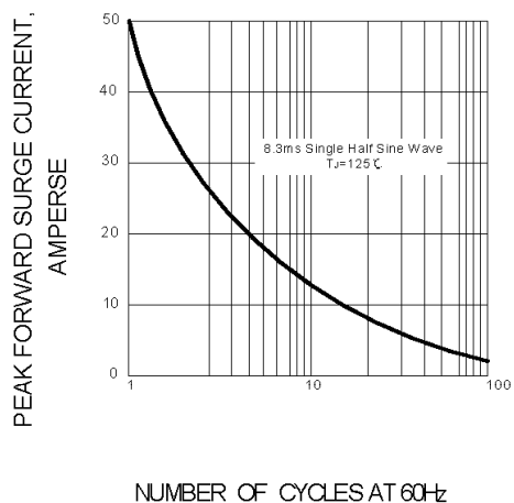
FIG.1 – PEAK FORWARD SURGE CURRENT
