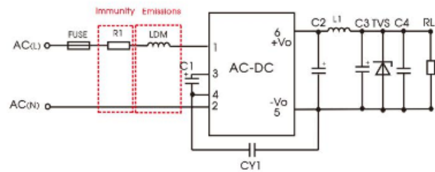
Recommended circuit 1
