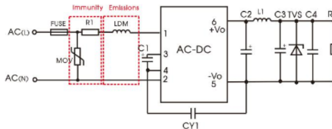
Recommended circuit 4
