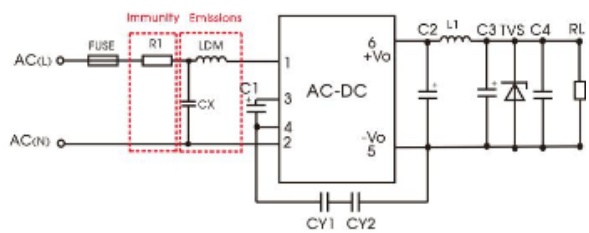
recommended circuit 2
