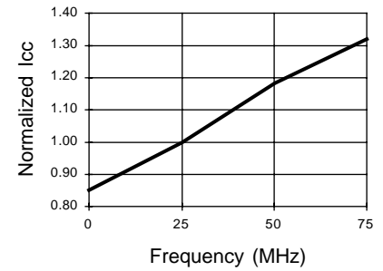
Normalized Icc vs Freq.
