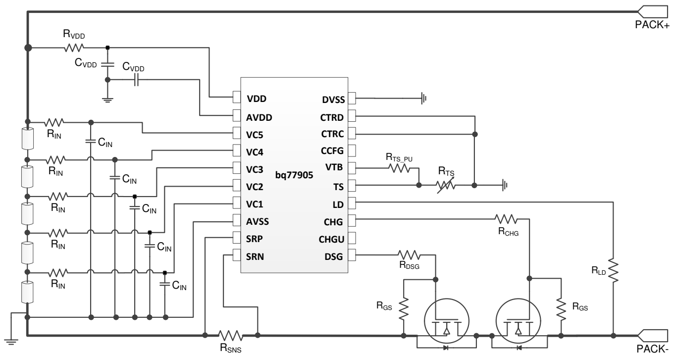
Figure 33. BQ77905 with Five Cells
