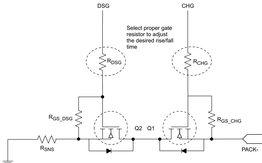
Figure 18. Select Proper Gate Resistor for FET Rise and Fall Time
