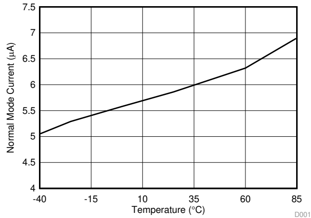
Figure 1. NORMAL Mode Current
