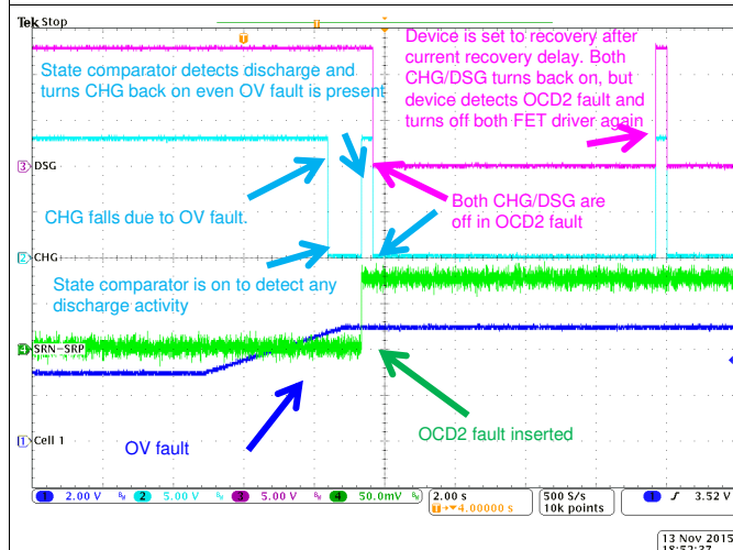
Figure 29. OV and OCD2 Faults Protection
