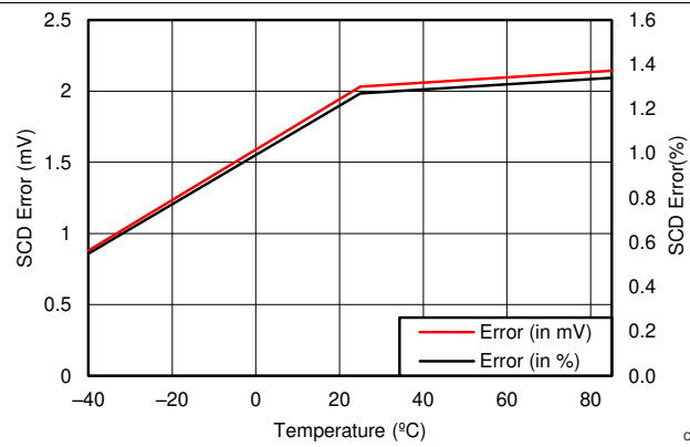
Figure 7. SCD Error at 160-mV Threshold
