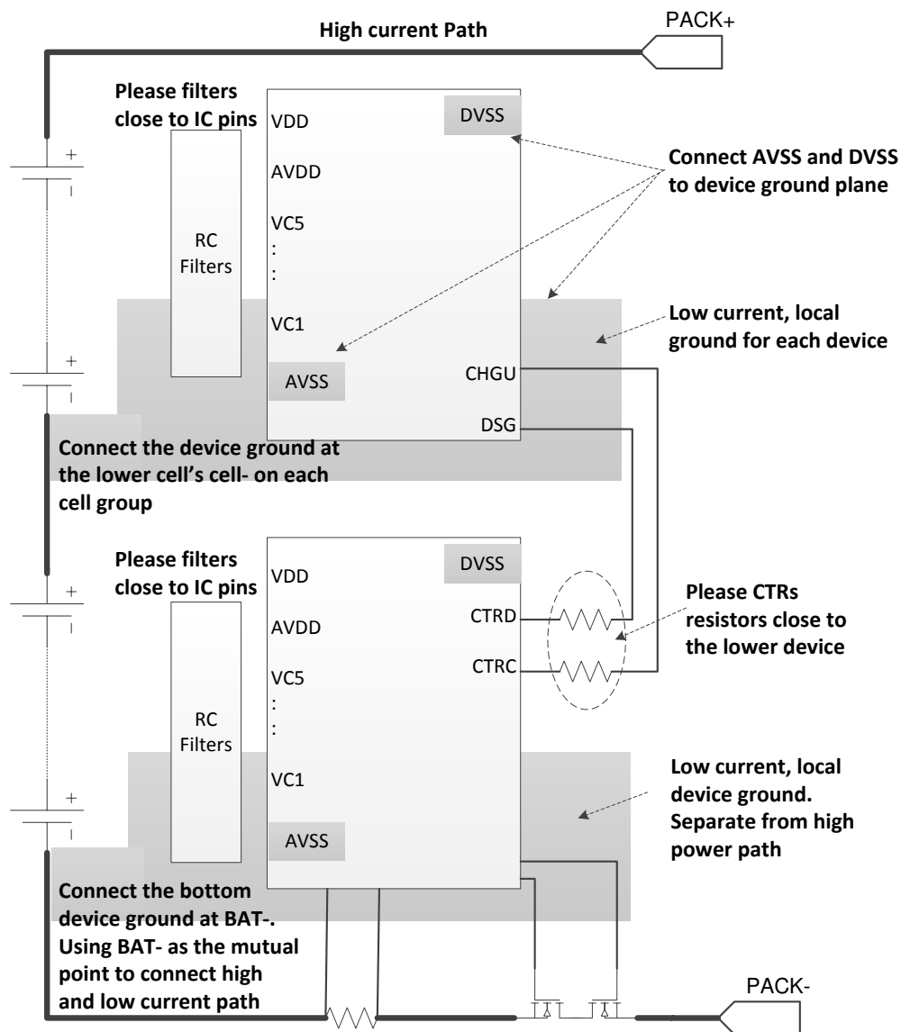
Figure 34. Layout Example
