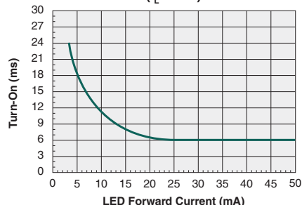
Typical Turn-On Time vs. LED Forward Current ( I_L=0.5\text{A} )
