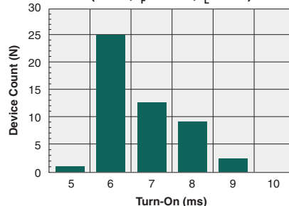
Typical Turn-On Time (N=50, I_F=10\text{mA} , I_L=0.5\text{A} )
