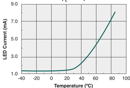
Typical I_F for Switch Operation vs. Temperature ( I_L=0.5\text{A} )
