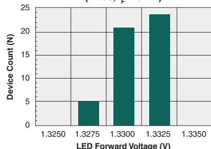
Typical LED Forward Voltage Drop (N=50, I_F=10\text{mA} )
