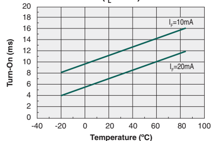
Typical Turn-On Time vs. Temperature ( I_L=0.5\text{A} )
