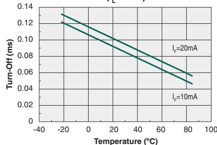
Typical Turn-Off Time vs. Temperature ( I_L=0.5\text{A} )
