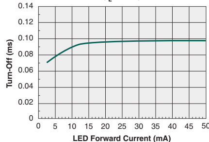
Typical Turn-Off Time vs. LED Forward Current ( I_L=0.5\text{A} )
