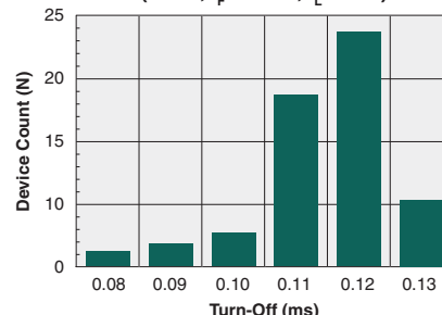
Typical Turn-Off Time (N=50, I_F=10\text{mA} , I_L=0.5\text{A} )
