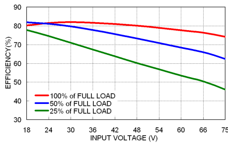
SDS(H)02-48S05W Efficiency vs. Input Voltage
