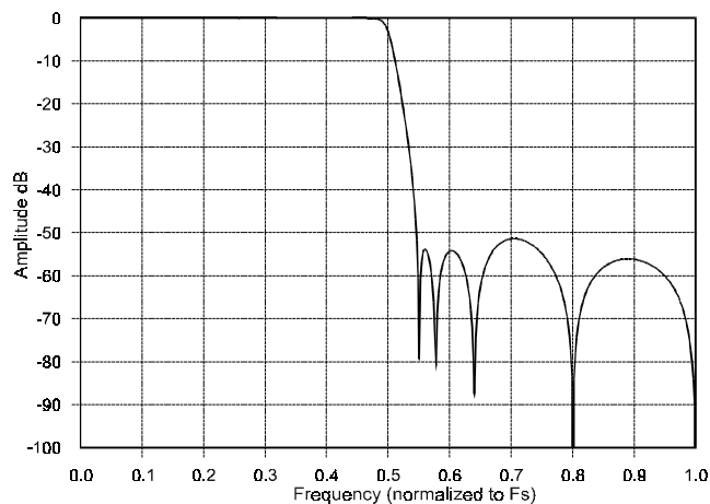
Figure 11. Single-Speed Stopband Rejection
