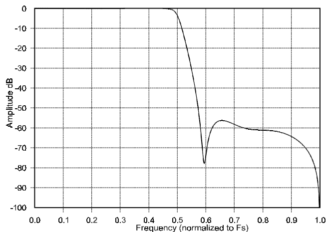
Figure 15. Double-Speed Stopband Rejection
