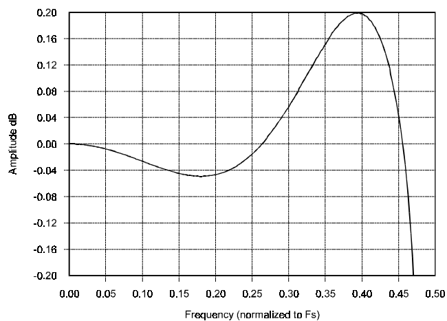
Figure 18. Double-Speed Passband Ripple
