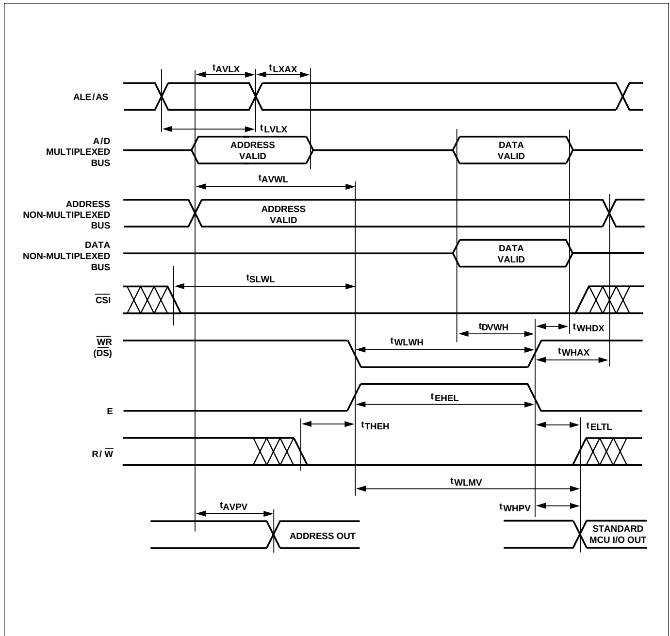
Figure 29. Write Timing
