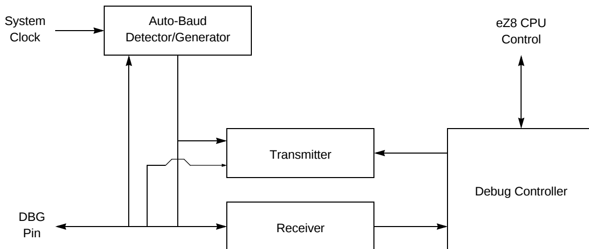
Figure 36. On-Chip Debugger Block Diagram
