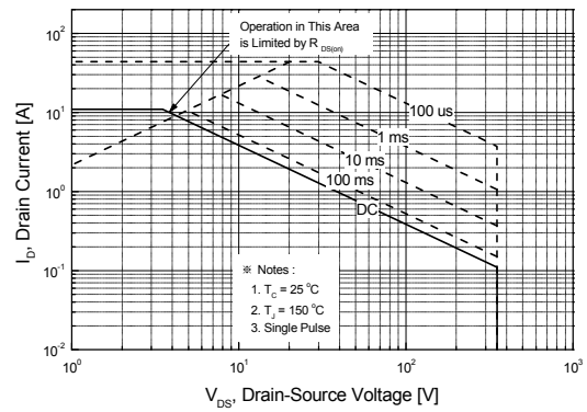
Figure 9-2. Maximum Safe Operating Area for SLF11N35UZ
