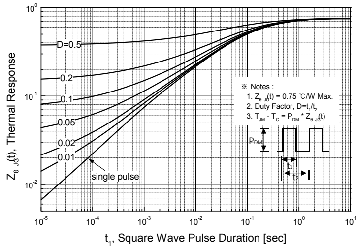
Figure 11-1. Transient Thermal Response Curve for SLP11N35UZ
