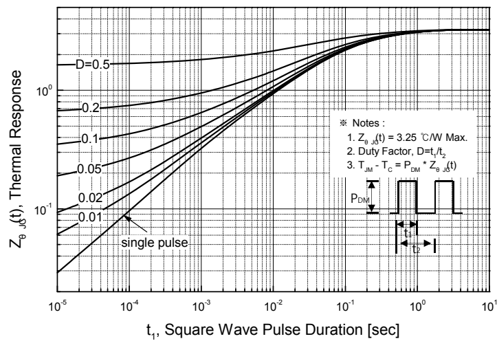
Figure 11-2. Transient Thermal Response Curve for SLF11N35UZ
