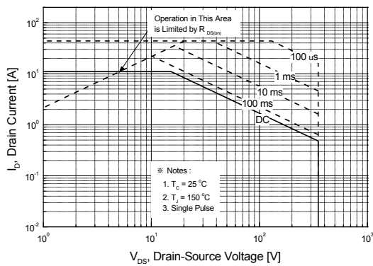
Figure 9-1. Maximum Safe Operating Area for SLP11N35UZ
