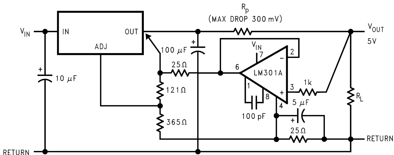
Figure 27. Remote Sensing
