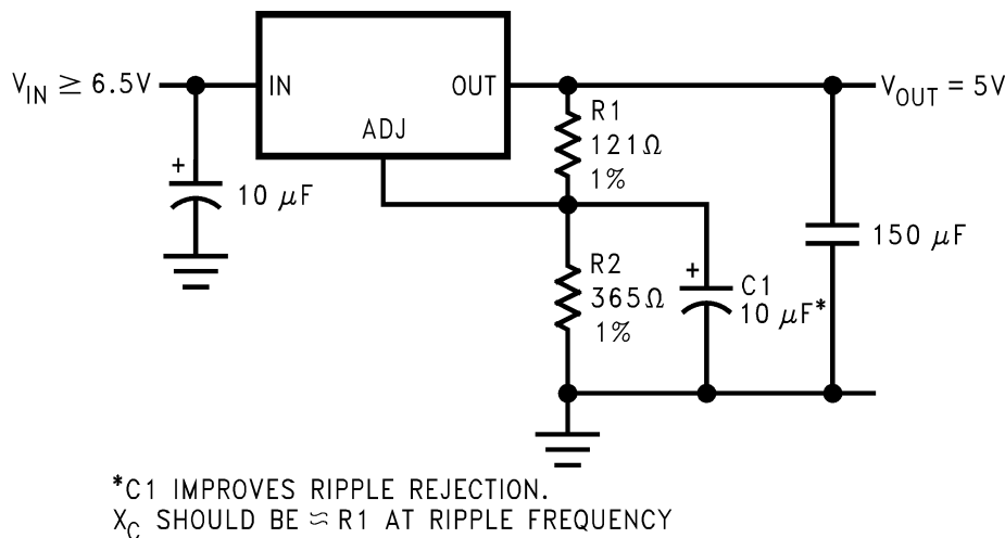
Figure 24. Ripple Rejection Enhancement
