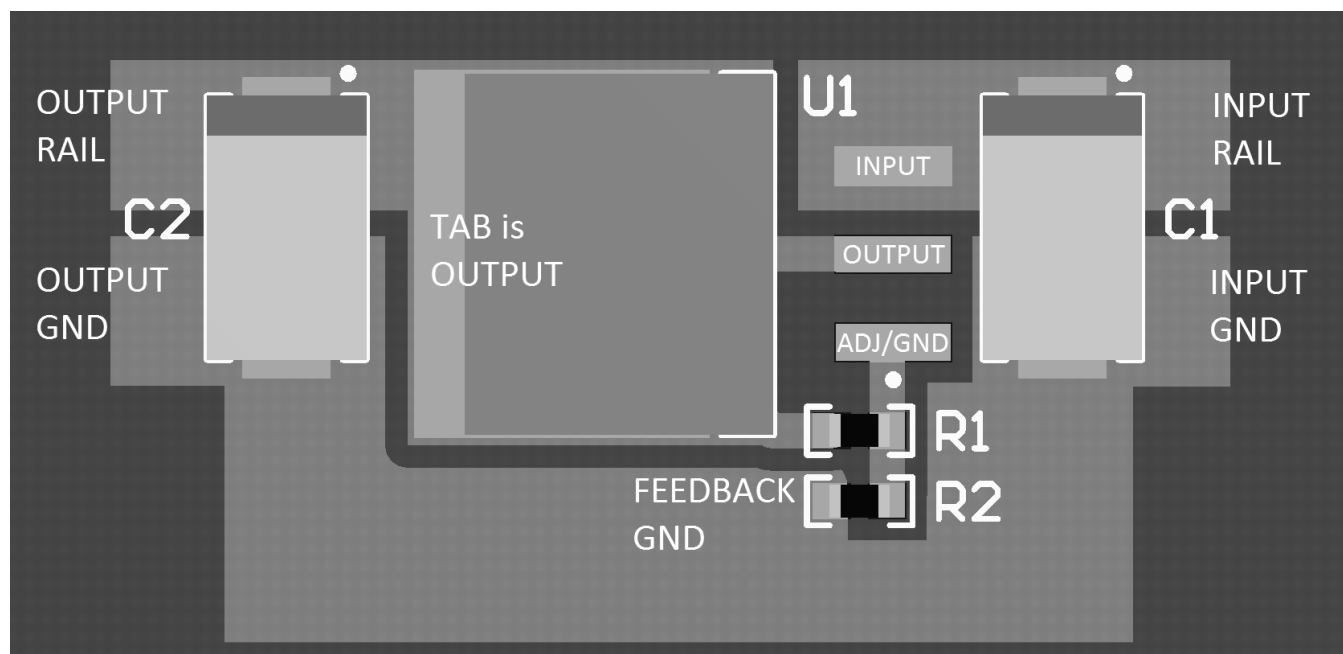
Figure 28. Layout Example
