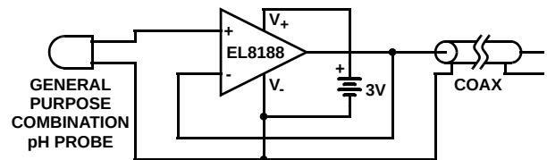
FIGURE 29. pH PROBE AMPLIFIER
