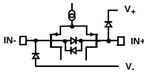
CIRCUIT 1
