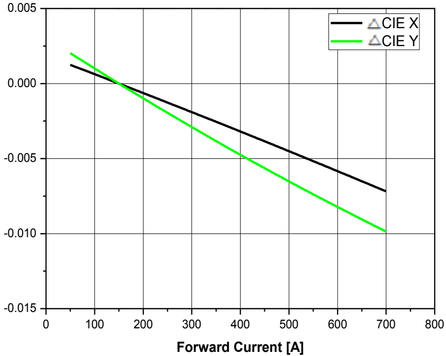
Fig 5. Forward Current vs. CIE X, Y Shift
