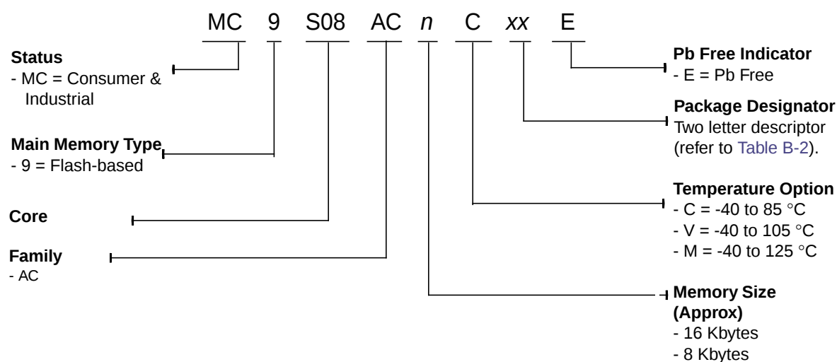
Figure B-1. Consumer &amp; Industrial Device Numbering System
