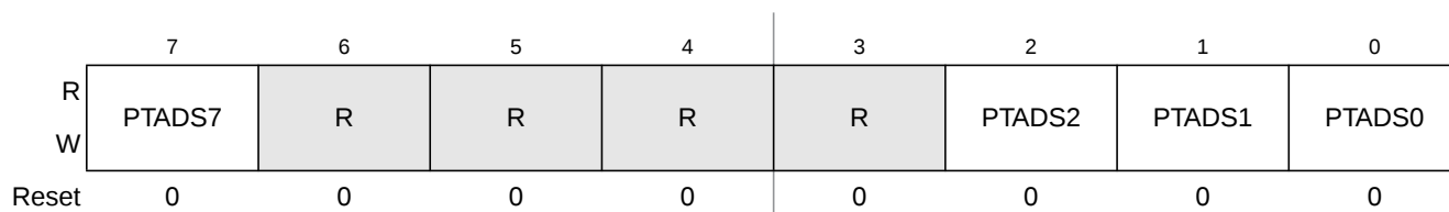
Figure 6-14. Internal Pullup Enable for Port A (PTASE) 1
