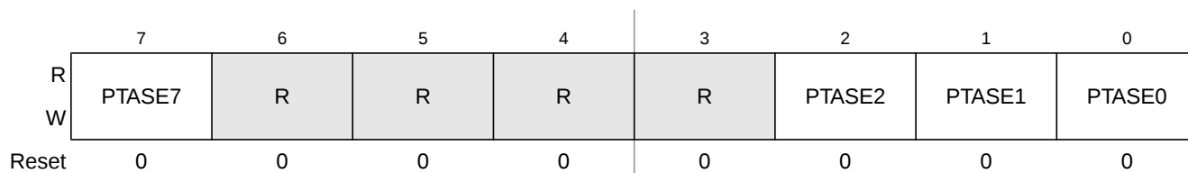
Figure 6-13. Internal Pullup Enable for Port A (PTASE) 1
