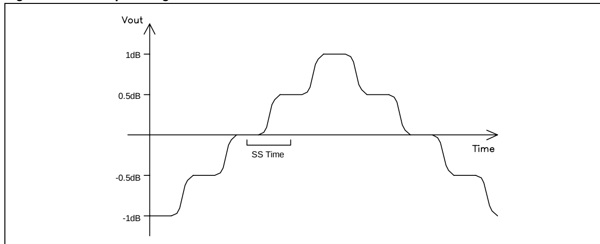
Figure 10. SoftStep-Timing
