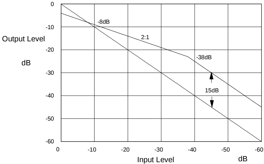
Figure 22. Compander Characteristic
