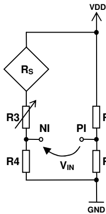
Figure 5. Temperature Measurement Configuration
