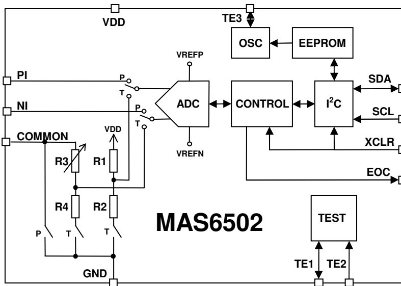
Figure 1. MAS6502 block diagram
