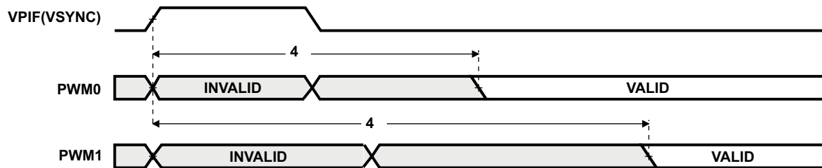
Figure 6-92. PWM Output Delay Timing
