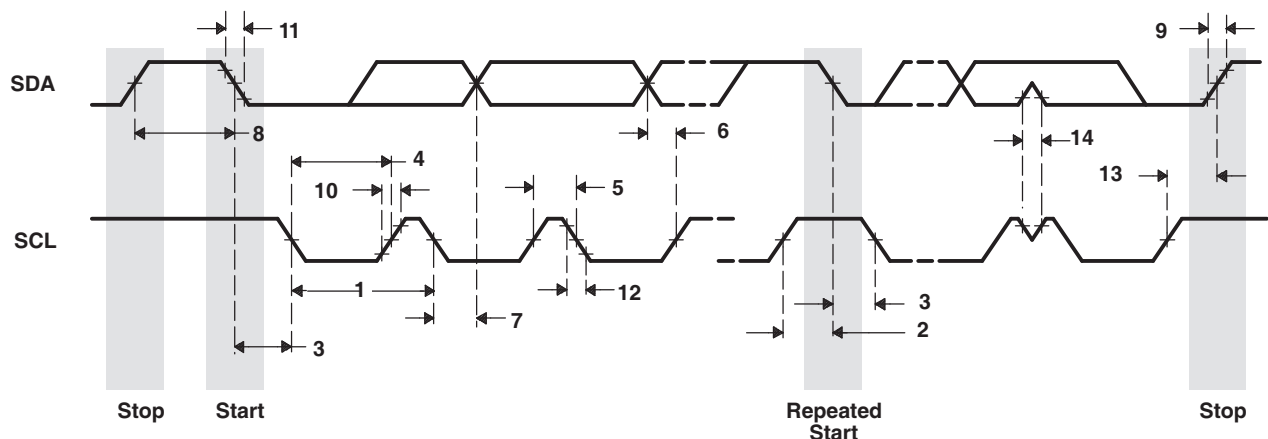
Figure 6-89. I 2 C Receive Timings
