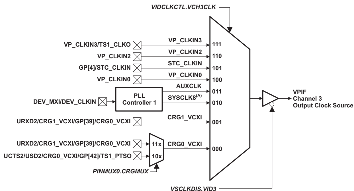
Figure 6-37. VPIF Display Channel 3 Source Clock Selection
