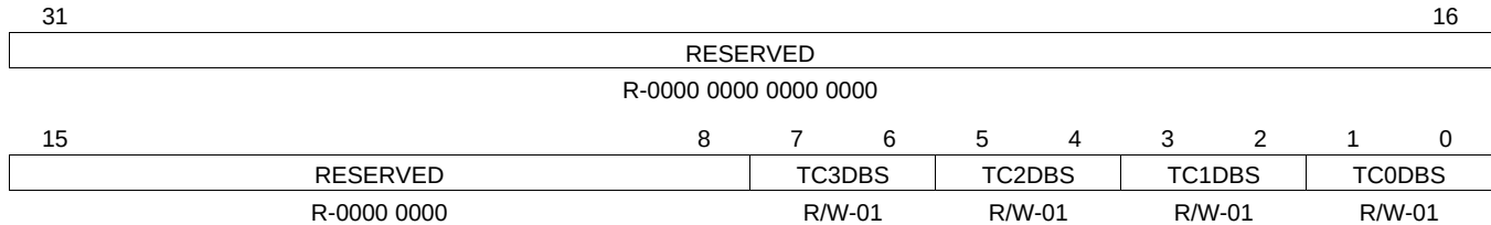
Figure 3-17. EDMA Transfer Controller Default Burst Size Configuration Register (EDMATCCFG) [0x01C4 0058]
