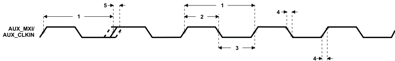
Figure 6-16. AUX_MXI/AUX_CLKIN Timing
