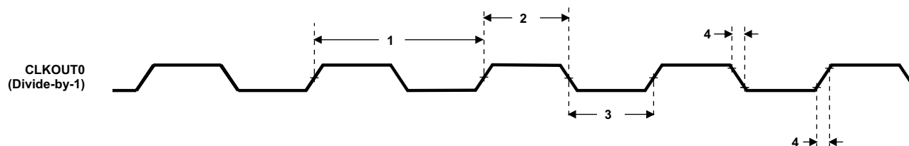
Figure 6-17. CLKOUT0 Timing
