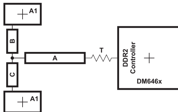
Figure 6-31. CK and ADDR_CTRL Routing and Topology
