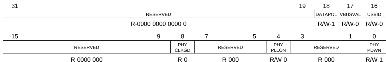
Figure 3-15. USBCTL Register [0x01C4 0034]
