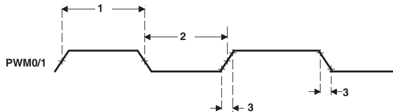
Figure 6-91. PWM Output Timing
