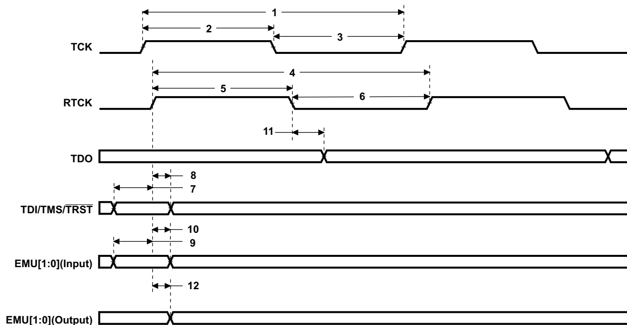
Figure 6-96. JTAG Test-Port Timing
