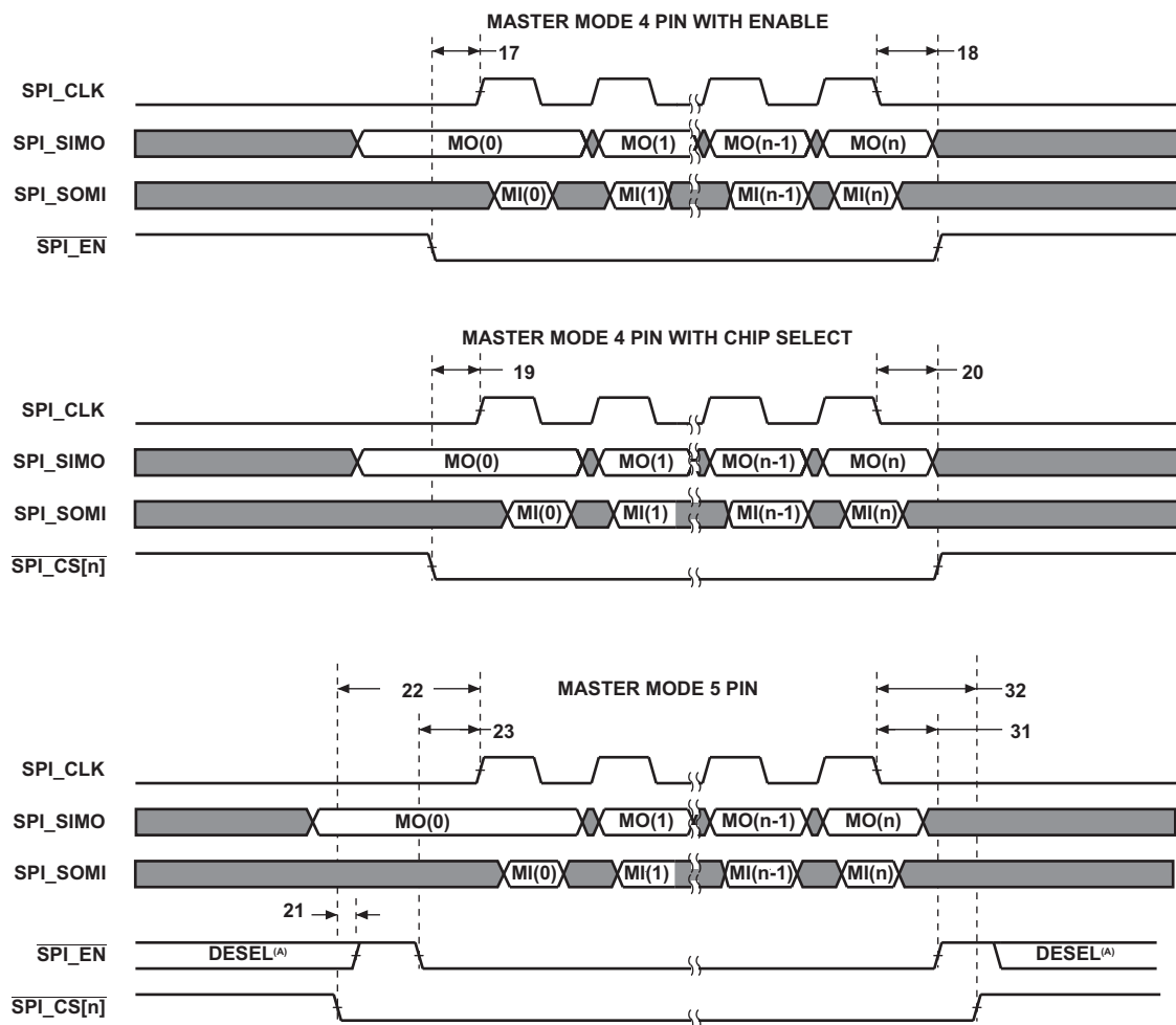
Figure 6-86. SPI Timings—Master Mode (4-Pin and 5-Pin)
