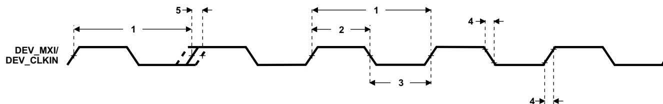
Figure 6-15. DEV_MXI/DEV_CLKIN Timing
