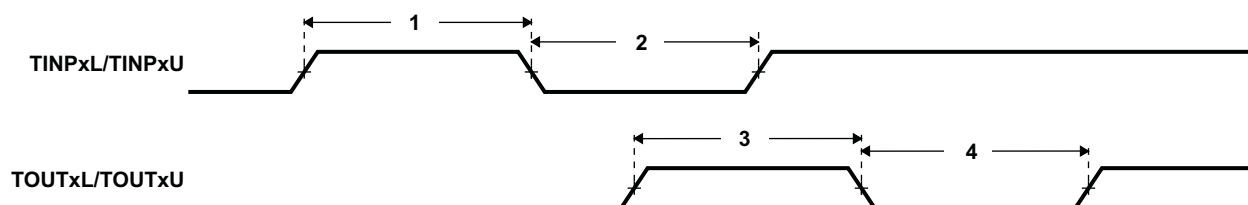
Figure 6-93. Timer Timing
