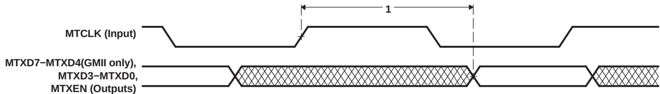
Figure 6-54. EMAC Transmit Interface Timing [MI and GMII Operation]
